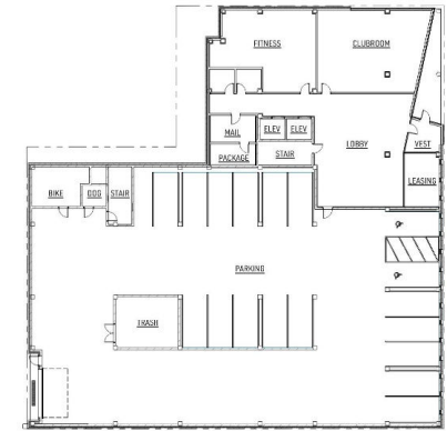
FLOOR PLAN - LEVEL 1 1/16" = 1'-0"
