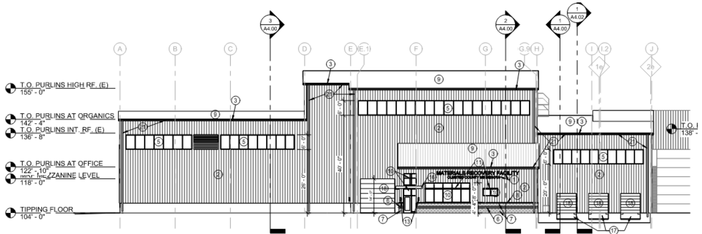
① MRF EAST ELEVATION 1/16" = 1'-0"
