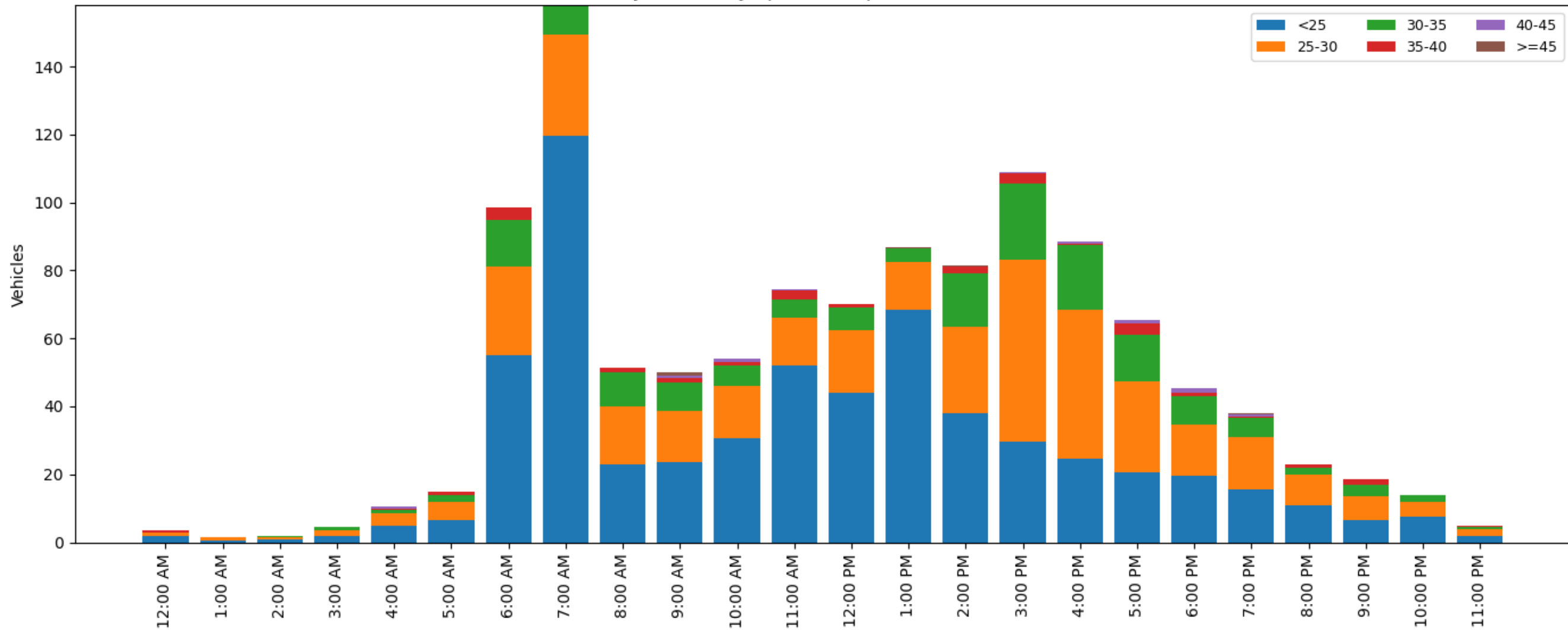
Hourly Volume by Speed Group at 1754 9th Ave SE
