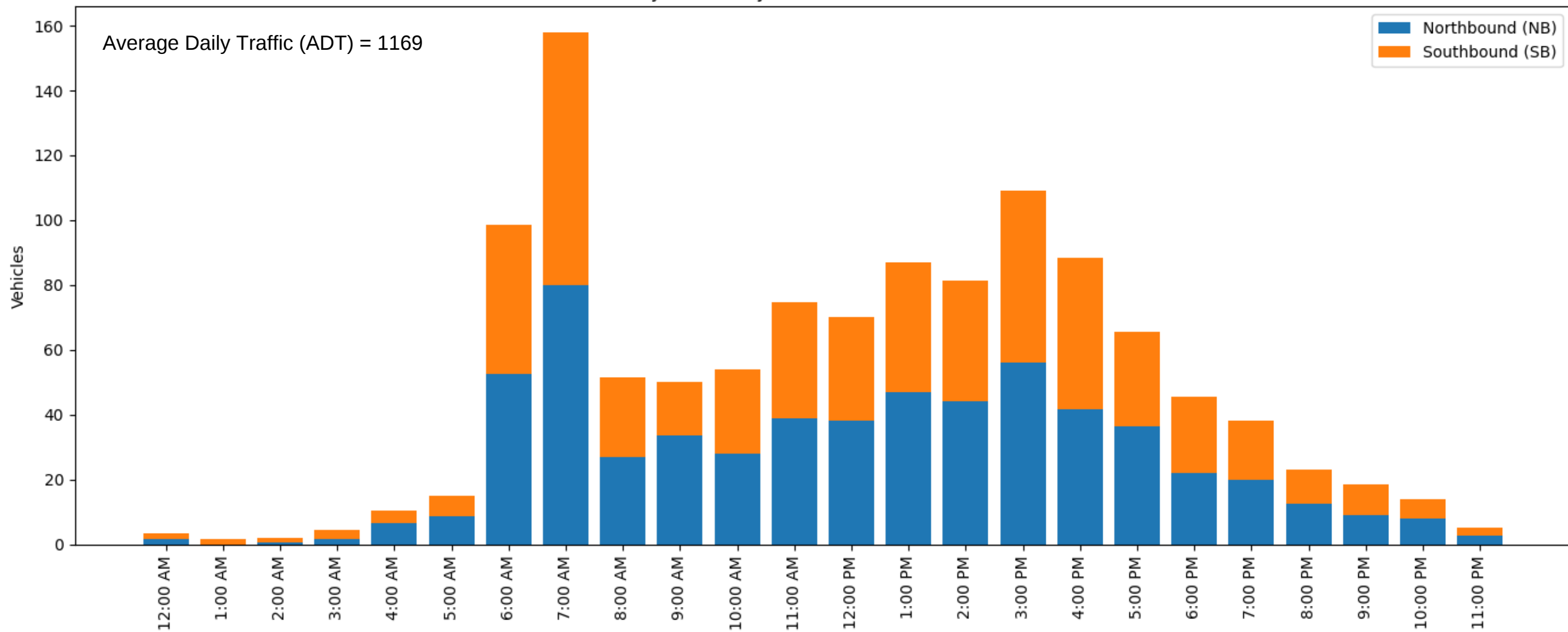
Hourly Volume by Direction at 1754 9th Ave SE
