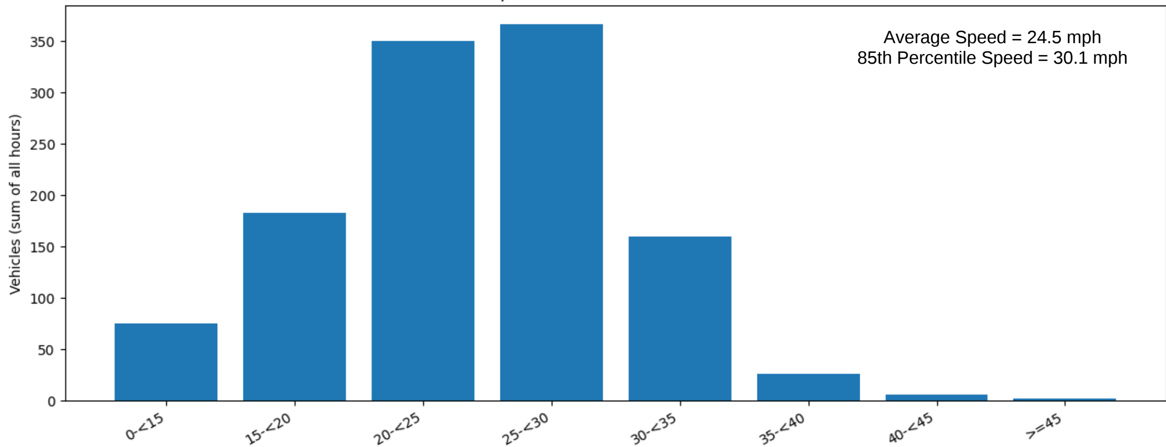
Overall Speed Distribution at 1754 9th Ave SE
