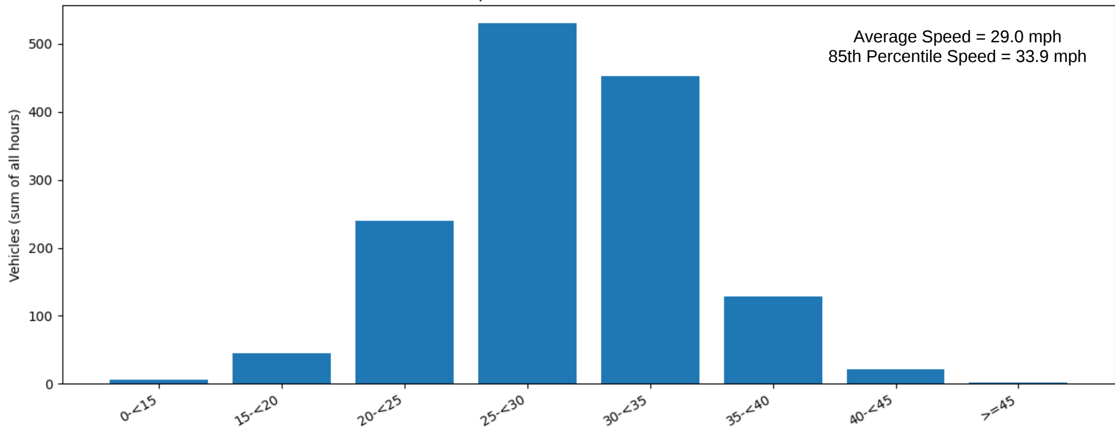
Overall Speed Distribution at 1641 9th Ave SE
